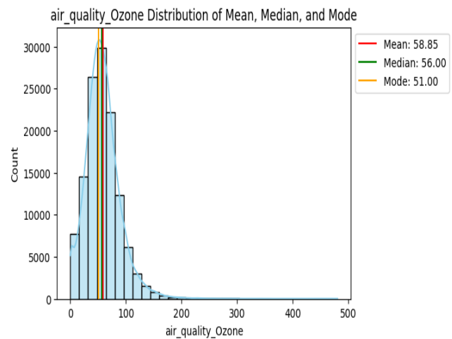
Figure 11: air_quality_Ozone
