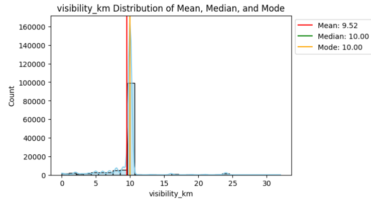
Figure 9: visibility_km
